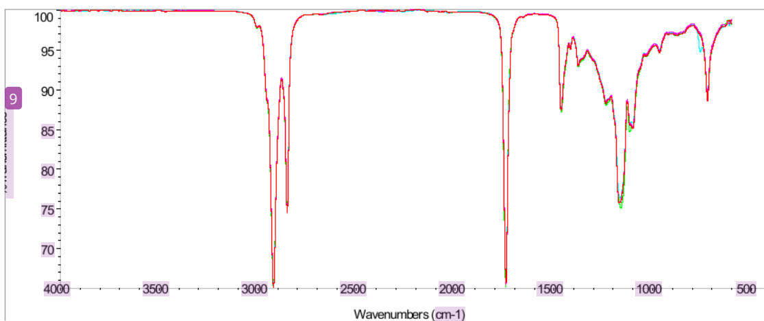
Figure 3: FTIR spectra of beef fat with four extraction method.
