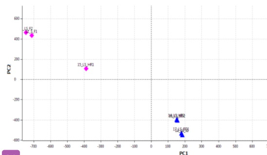
21 Figure 1: The score plot of PCA model using fatty acid composition of beef fat in SO, FO, BD, and HR.
