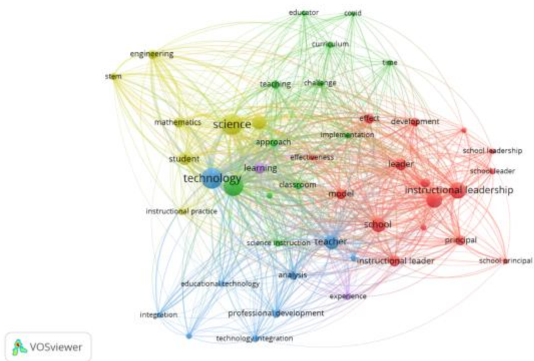
Figure 2. Network Vizualitation
