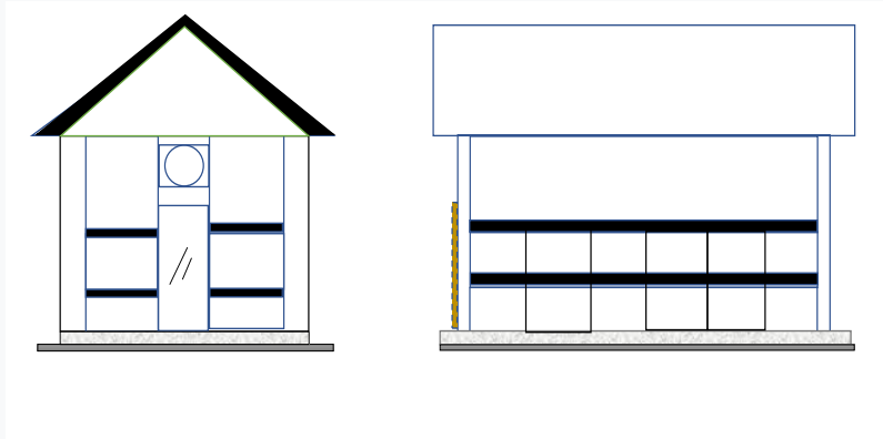
Figure 1. Prototype of FRP house model of straw mushroom (Dimentions 3,0 m x 5,0 m x 3,0 m)
