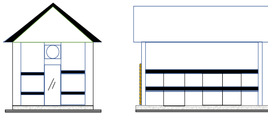
Figure 1. Prototype of FRP house model of straw mushroom (dimentions 3.0 m x 5.0 m x 3.0 m)
