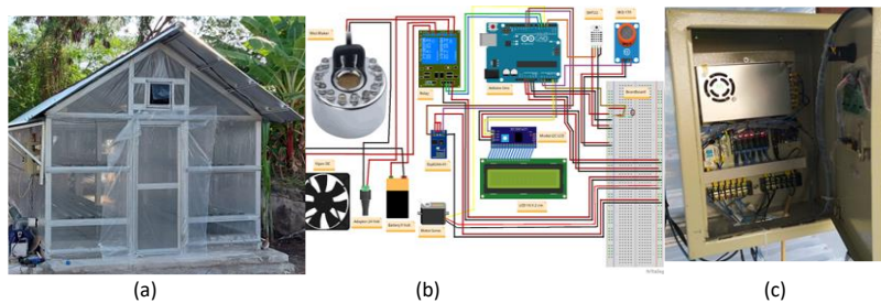
Figure 3. The prototype of the FRP house (a) with IoT circuit (b) and panel control box (c)
