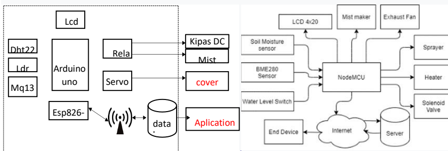
Figure 2. Architecture of IoT of production house in oyster mushroom
