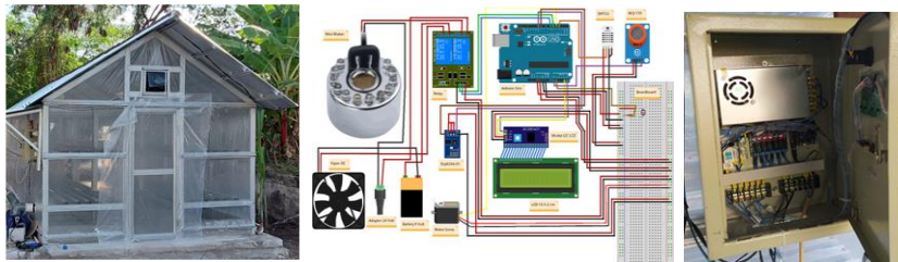
Figure 3. The prototype of the FRP house with IoT circuit
