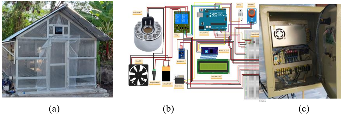
Figure 3. The prototype of the FRP house (a) with IoT circuit (b) and panel control box (c)
