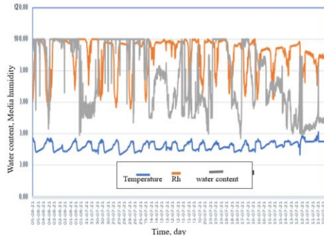
Figure 4. Fluctuation of air temperature, RH, and moisture content inside FRP House
