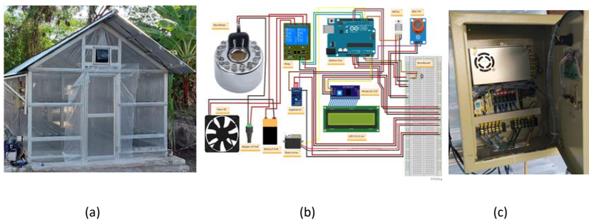
Figure 3. The prototype of the FRP house (a) with IoT circuit (b) and panel control box (c)
