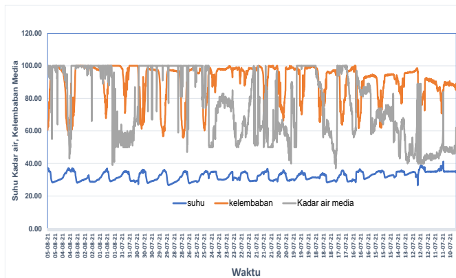
Figure 4. Condition of air temperature, RH, and moisture content inside FRP House
