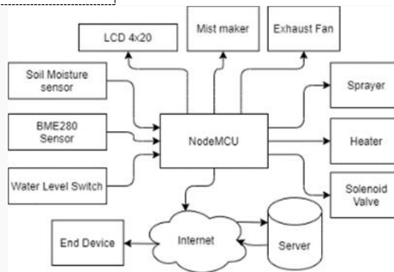
Figure 2. Architecture of IoT of production house in oyster mushroom
