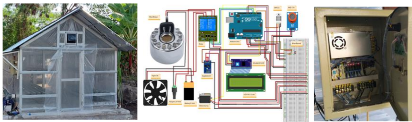
Figure 3. The prototype of the FRP house with IoT circuit
