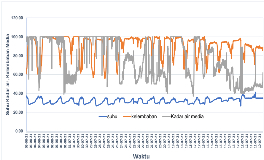
Figure 4. Fluctuation of air temperature, RH, and moisture content inside FRP House
